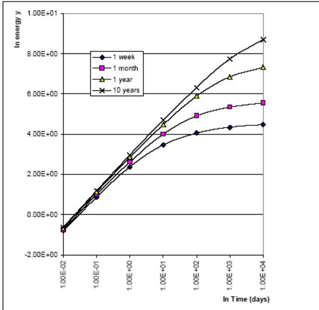
Figure 6. Decay energy release after shutdown for a 3,000 MWth PWR for different operational times.
